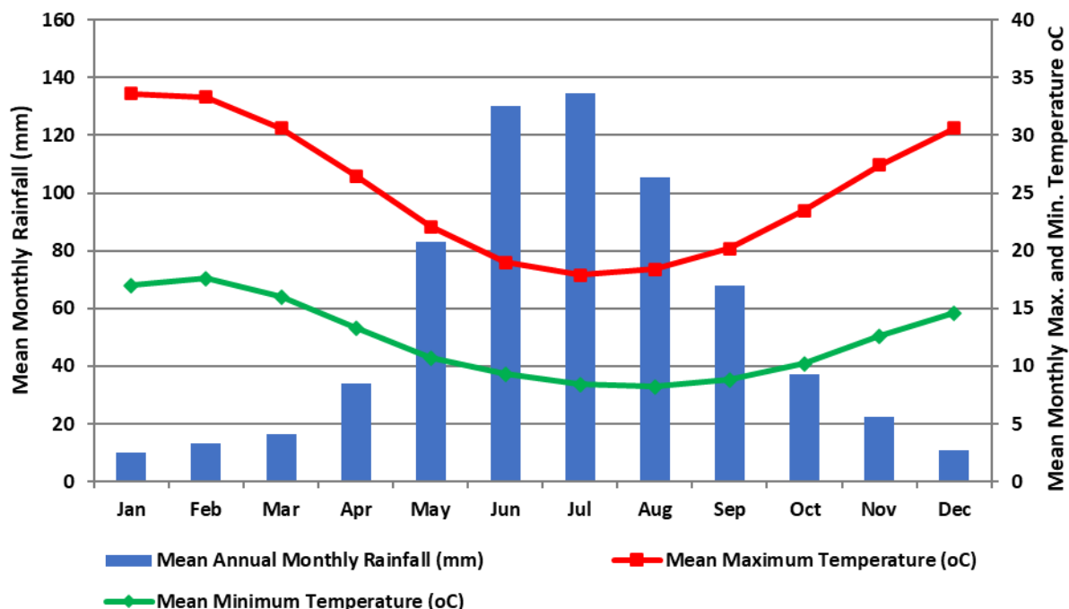
Figure 2: Summary of Climatic data from Bureau of Meteorology (BOM 2022) for the Pearce RAAF Airbase 009053 (Rainfall, Minimum and Maximum Temperatures °C)
