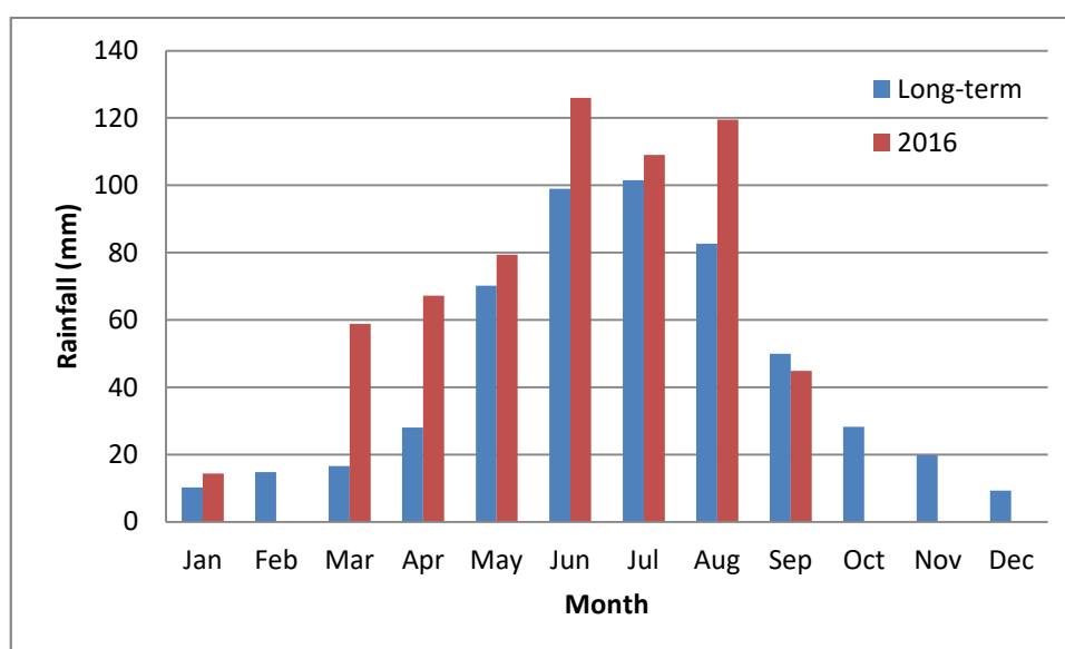
Figure 2.1: Rainfall for Badgingarra – long-term and 2016 Source: Bureau of Meteorology Climate Data Online (1962 to 2016)
