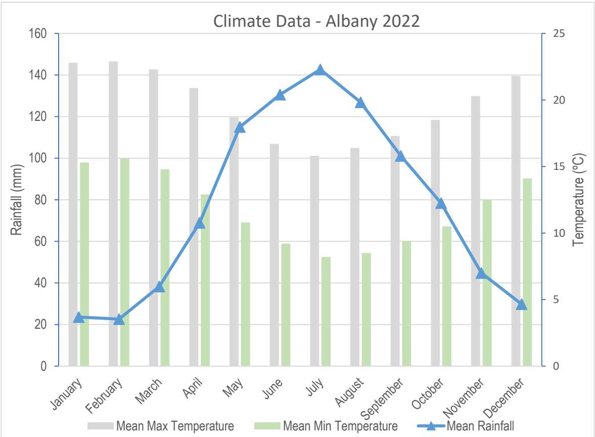
Figure 2. Climate data recorded at Albany City Weather Station (Rainfall and maximum temperature 12 months prior to survey and long-term average) (Bureau of Meteorology 2023).
