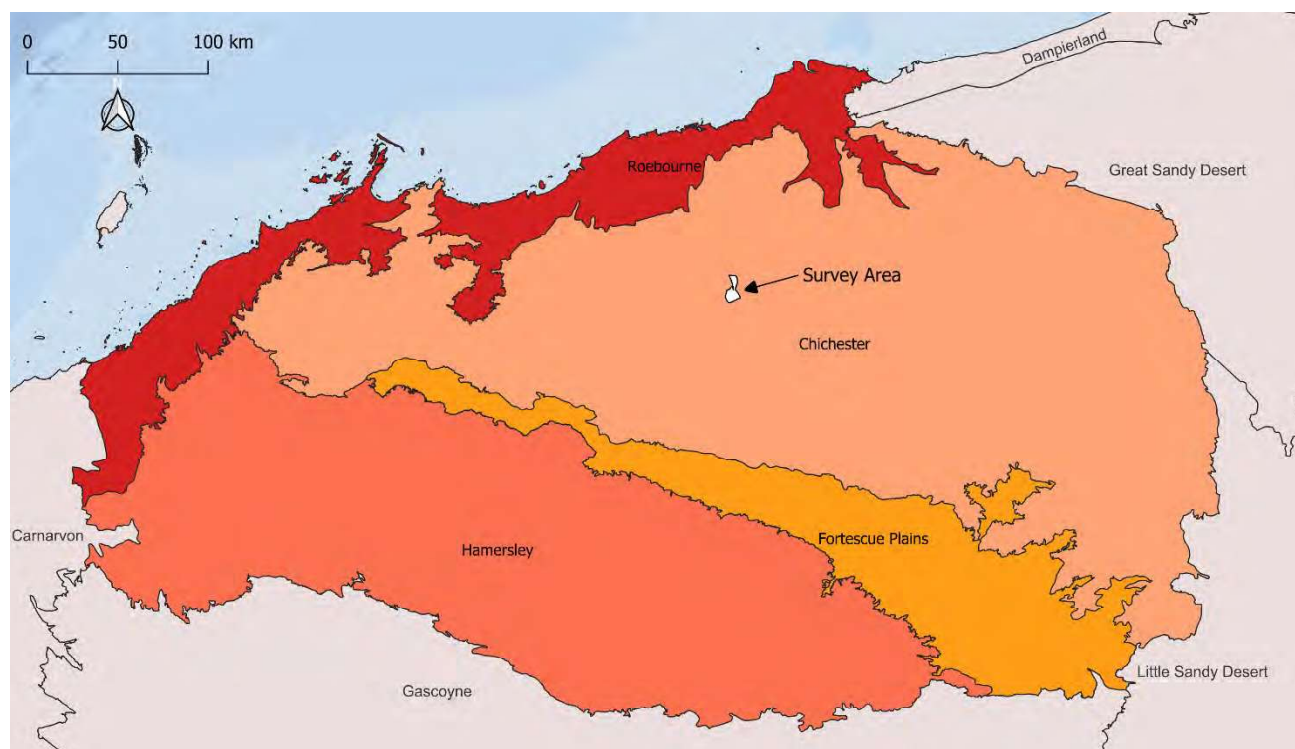
Figure 2.1: IBRA Classification
