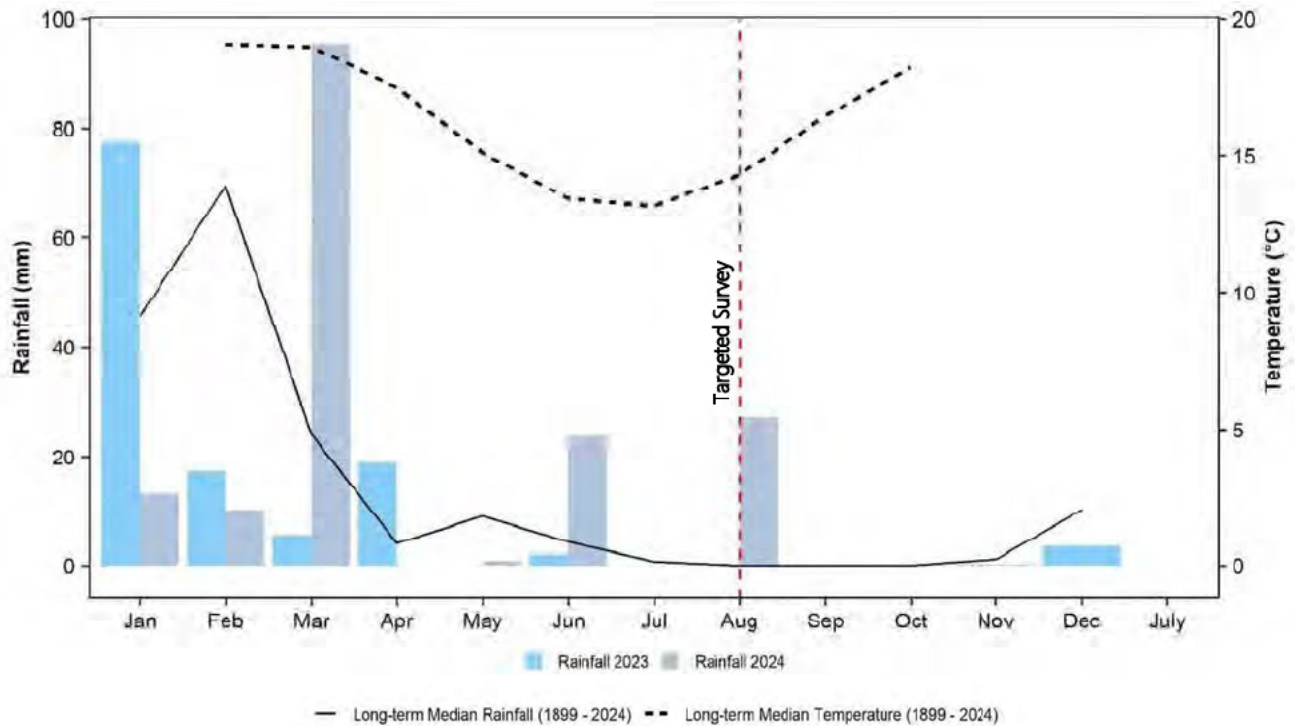
Figure 3.1: Rainfall Data at SILO Request Location (-21.2066, 118.7585).
