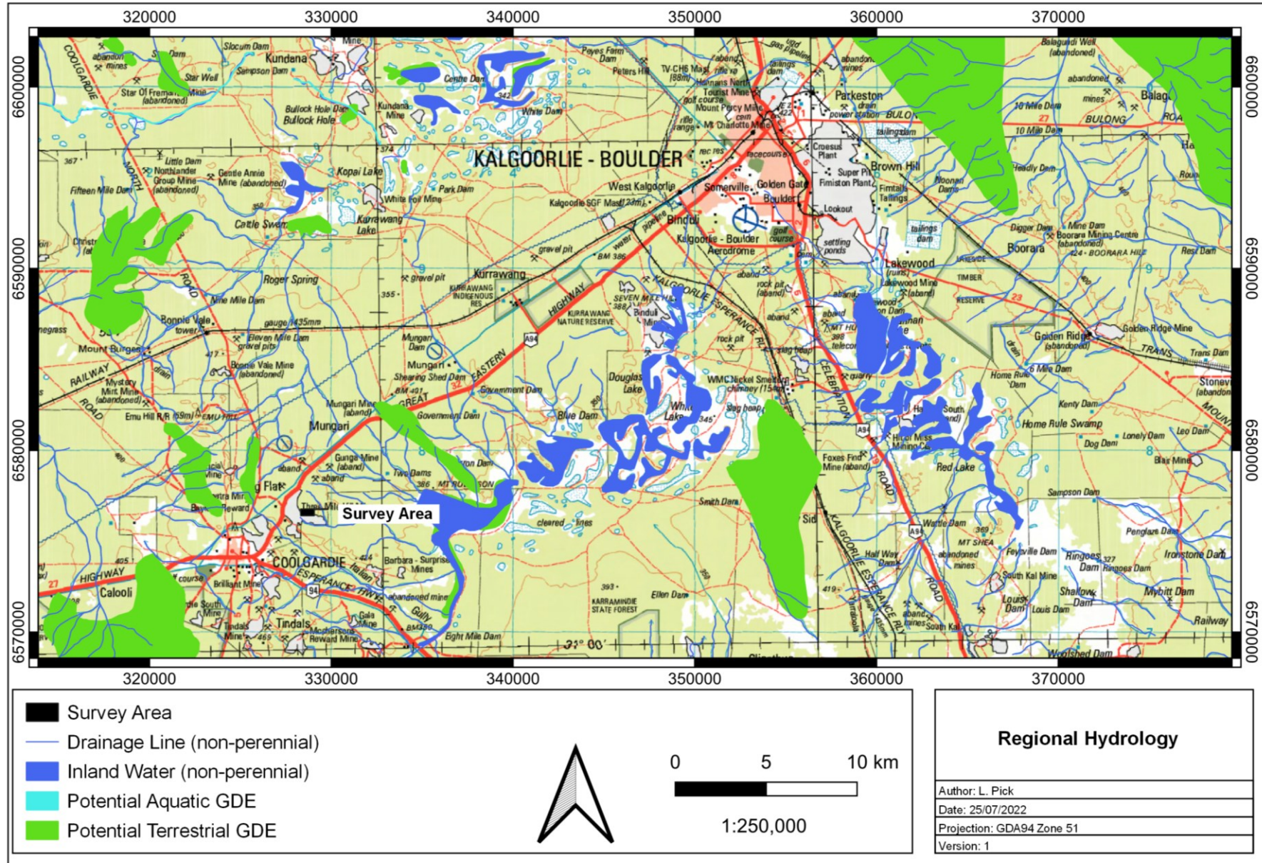
Figure 2-4: Regional Hydrology
