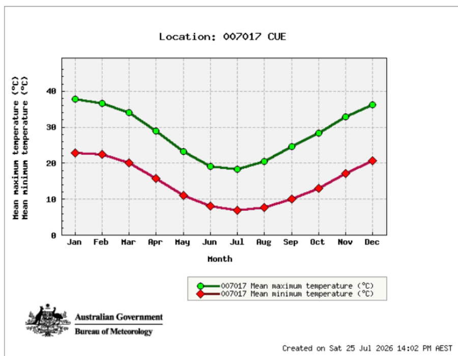
Figure 2: Mean temperature ranges for Cue weather station
