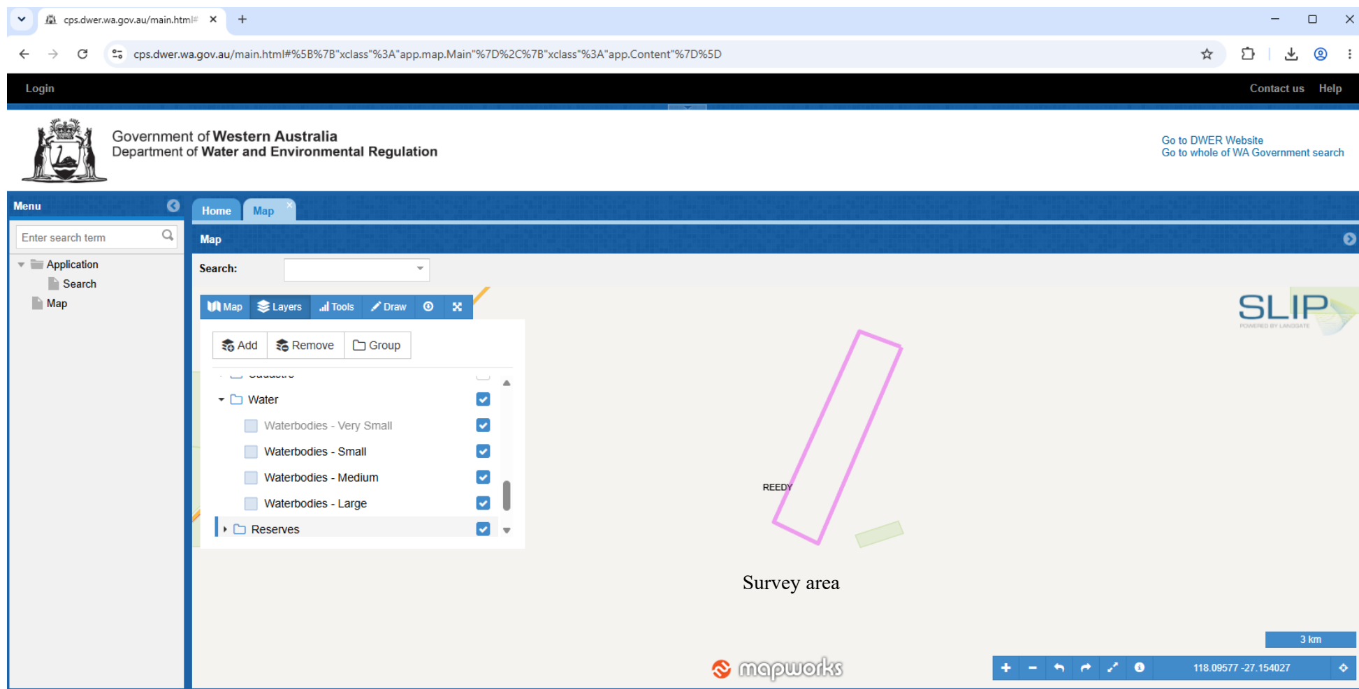
DWER Clearing Permit System Map Viewer showing no waterbodies within the survey area (DWER, 2026)
