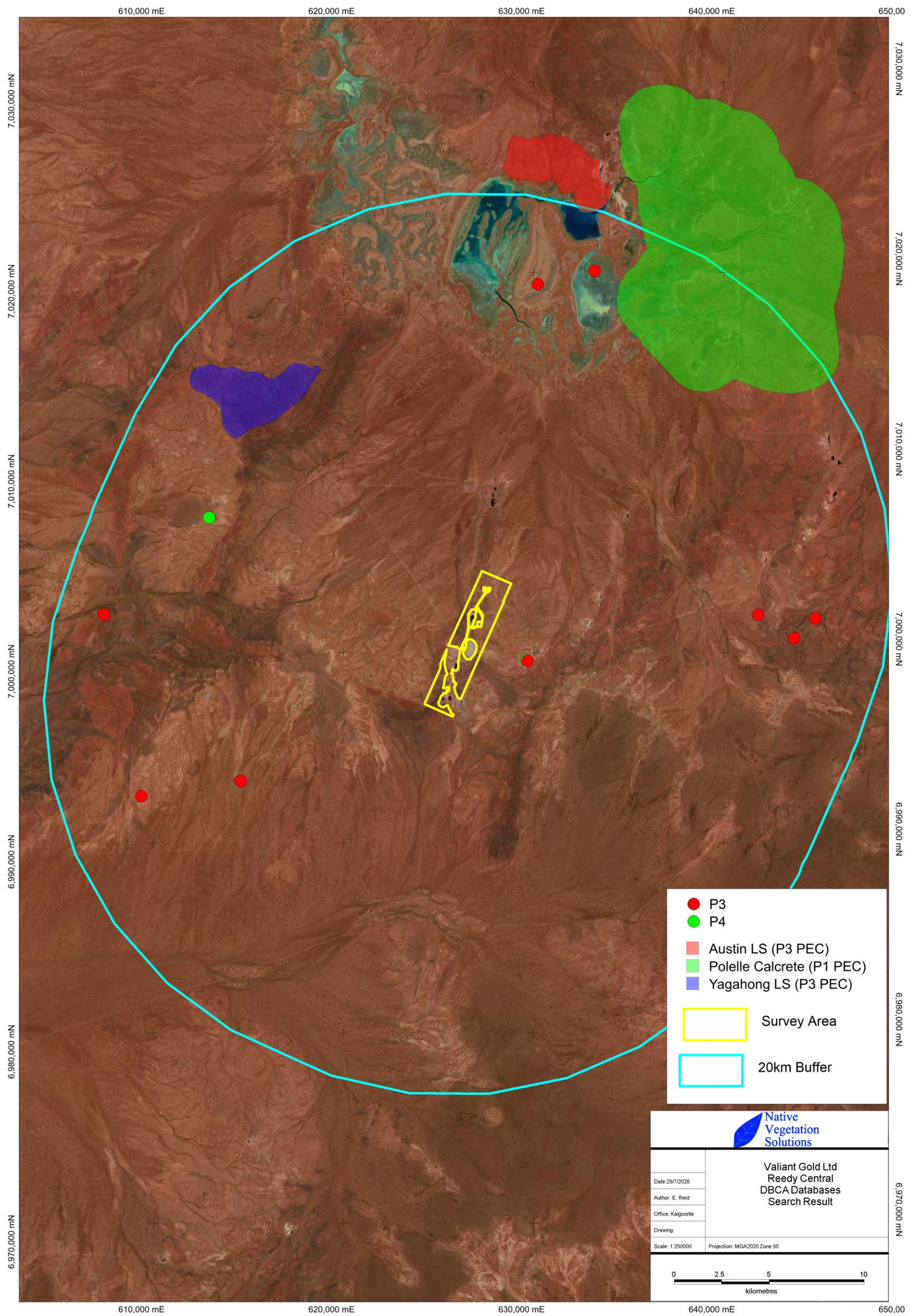
Map 3: DBCA Databases Search Results
