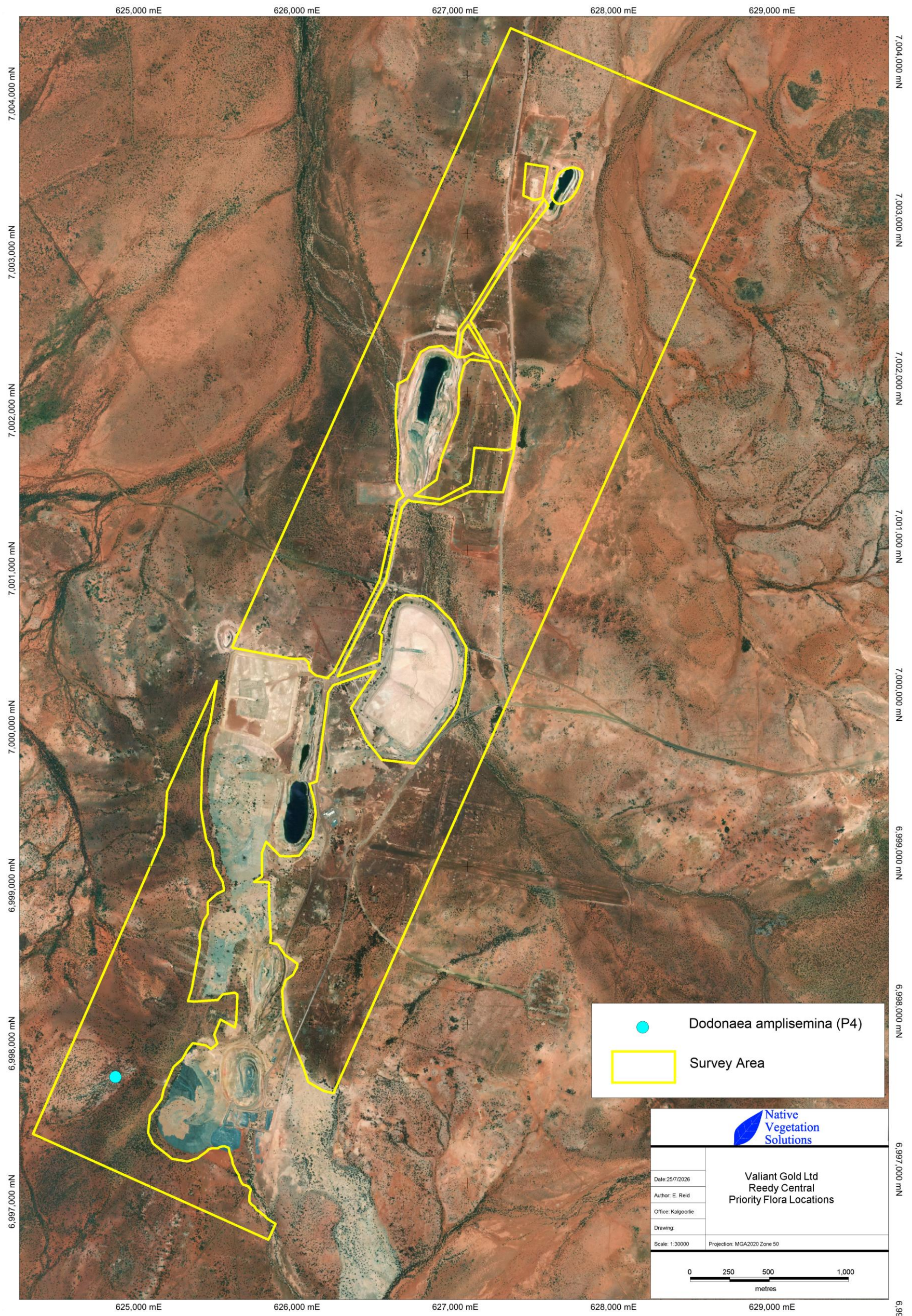
Map 8: Priority Flora Locations
