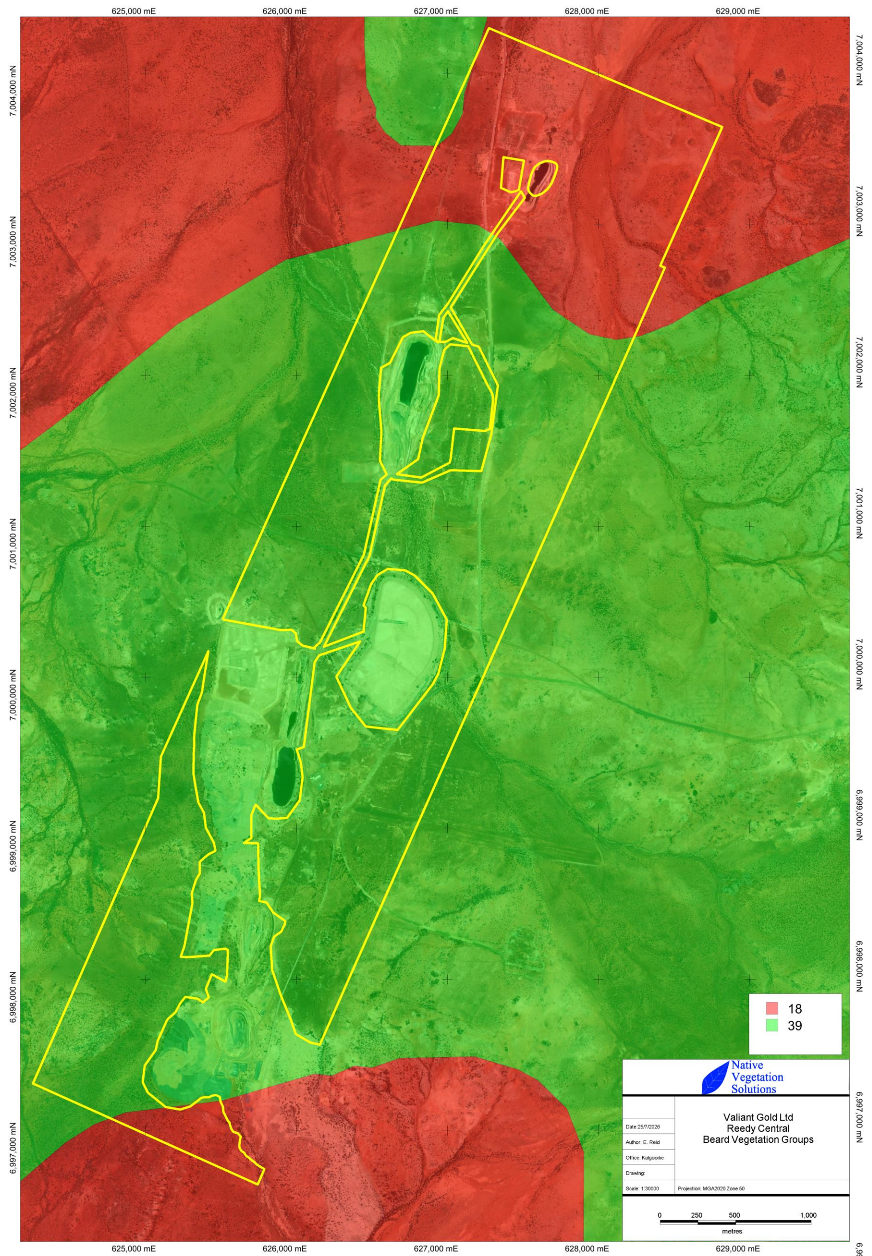
Map 5: Beard Pre-European Vegetation Groups
