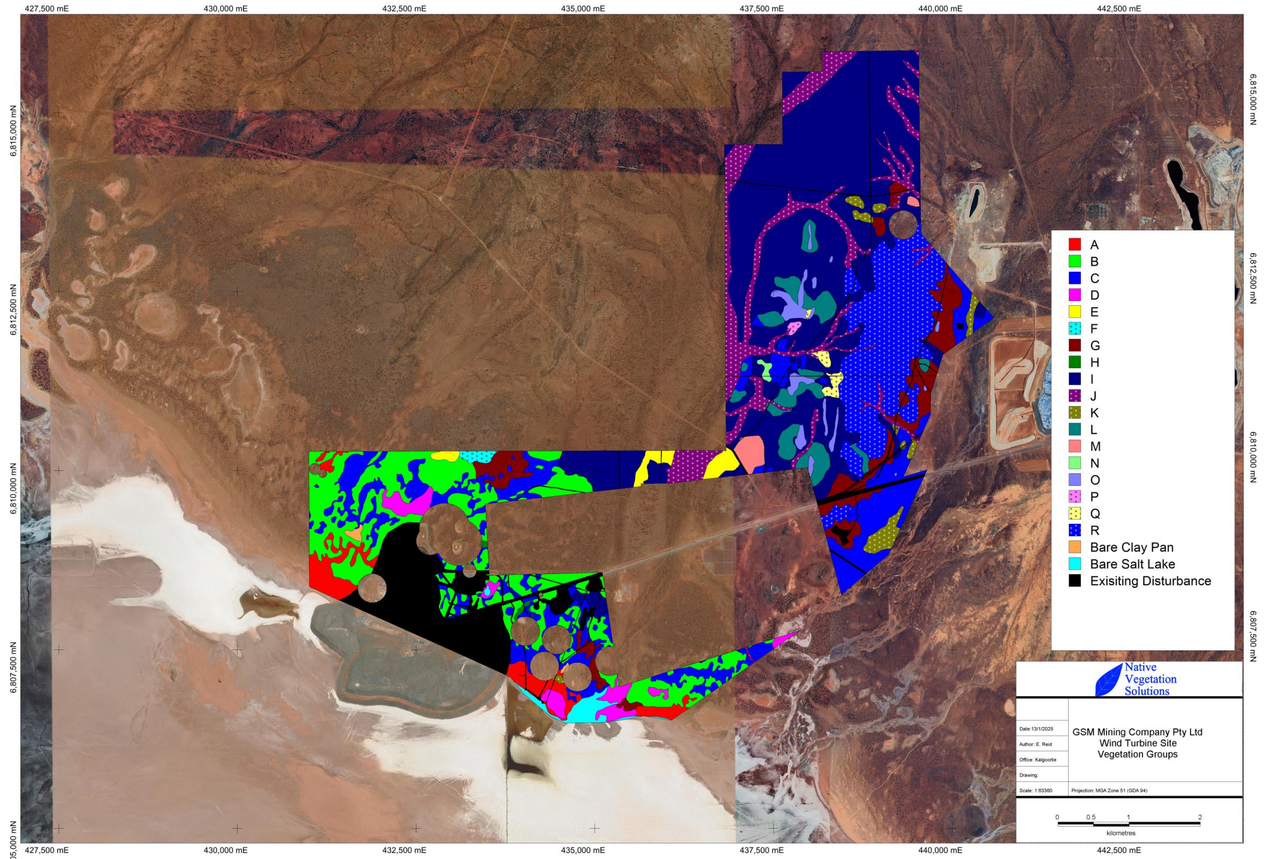
Map 5: Vegetation Groups
