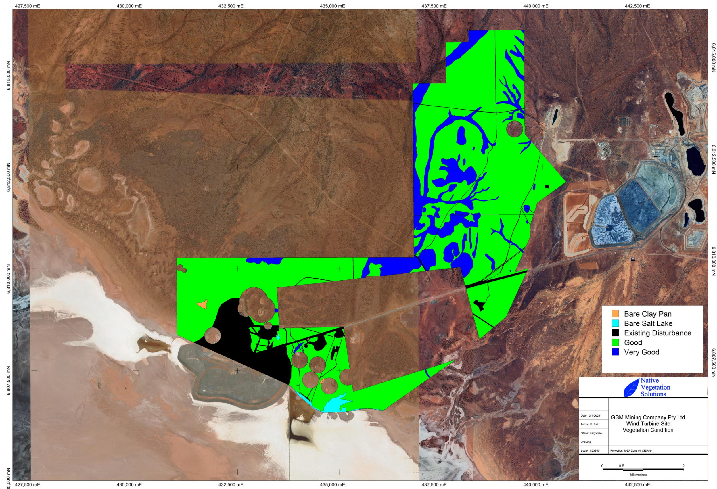
Map 6: Vegetation Condition
