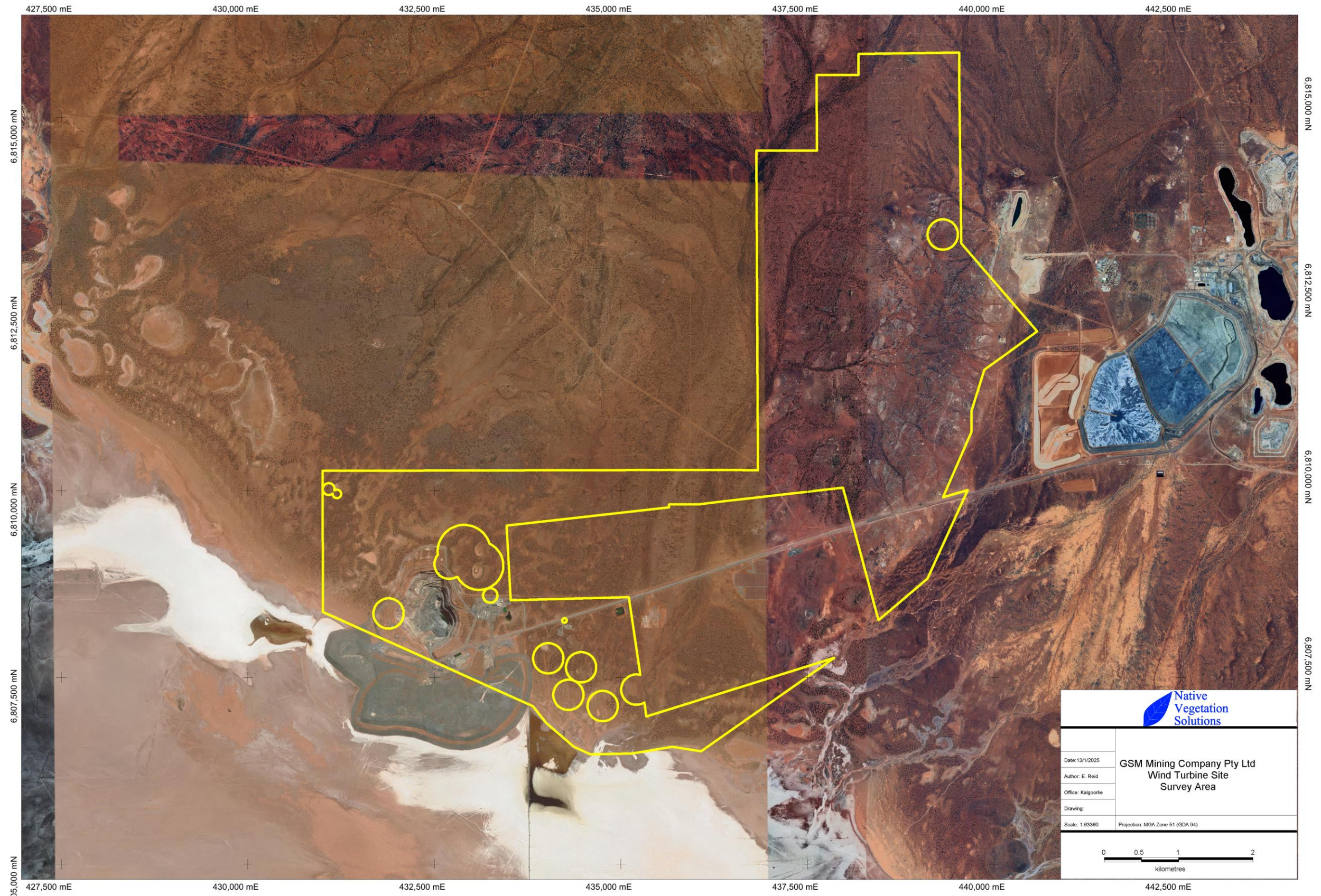
Map 1: Survey Area
