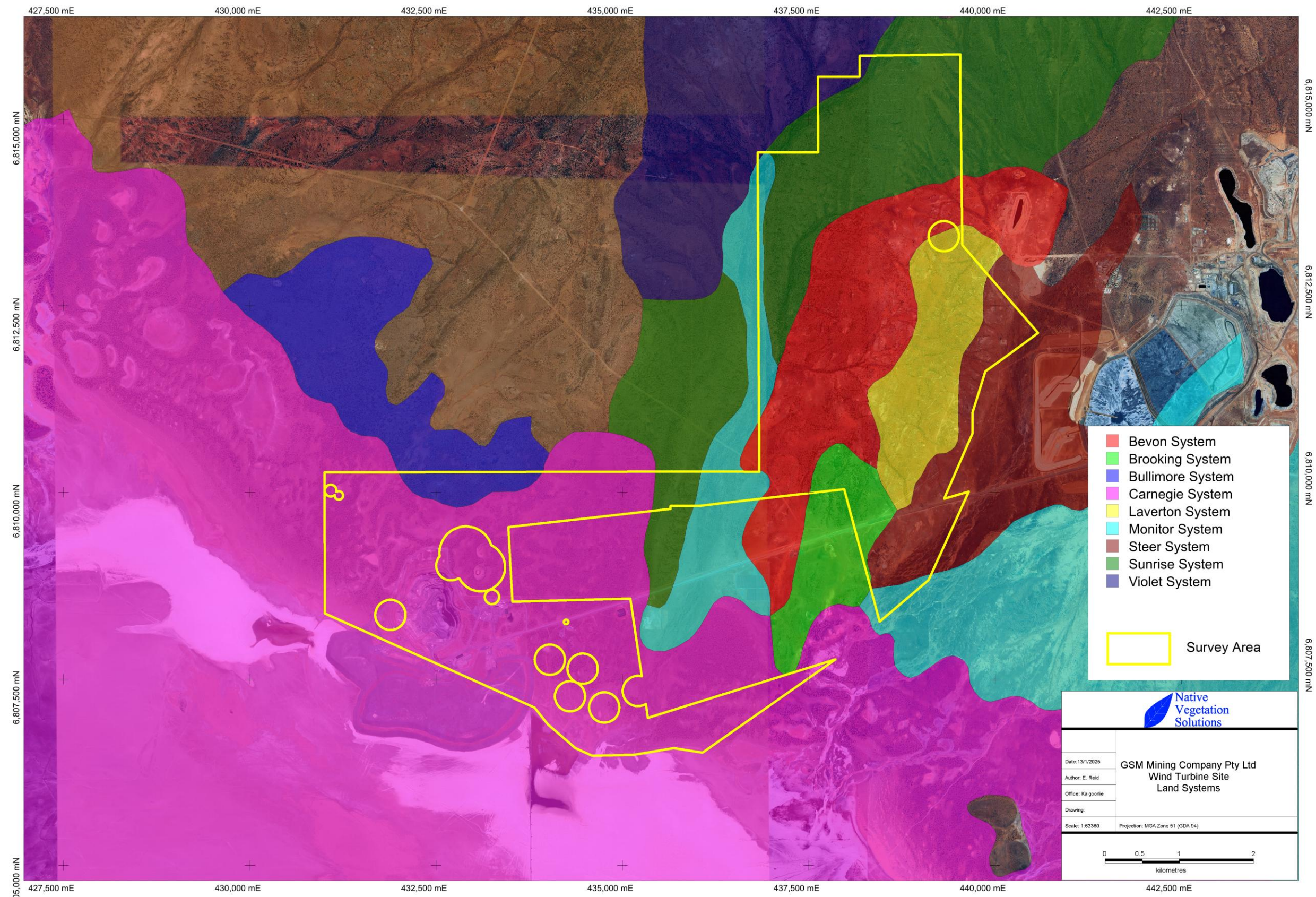
Map 4: Land Systems
