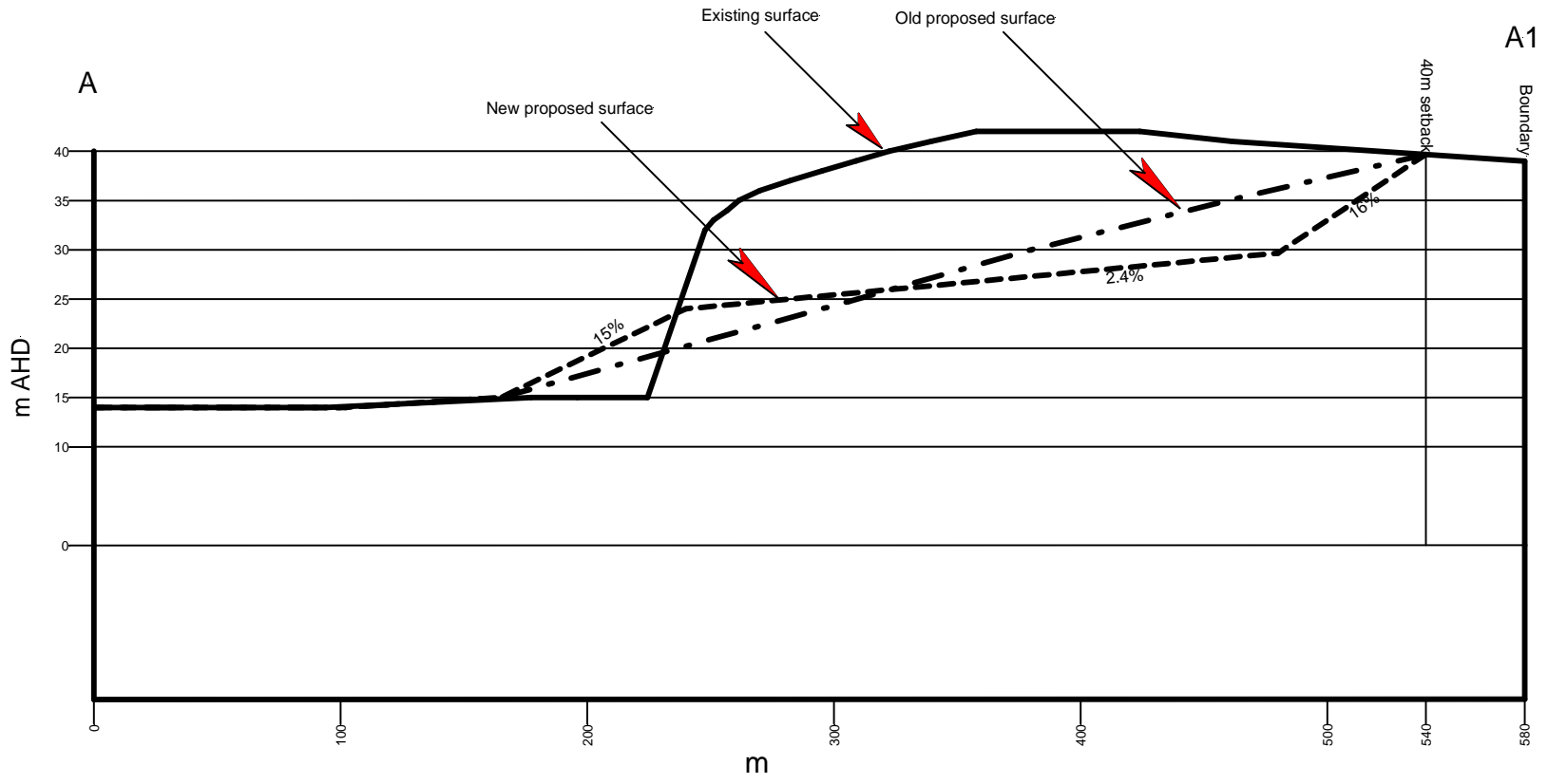
FIGURE 5 Lot 520 and Boyanup AA 187, Bussell Highway, Stratham B&J Catalano Pty Ltd Long Section A - A1 VE=4x
