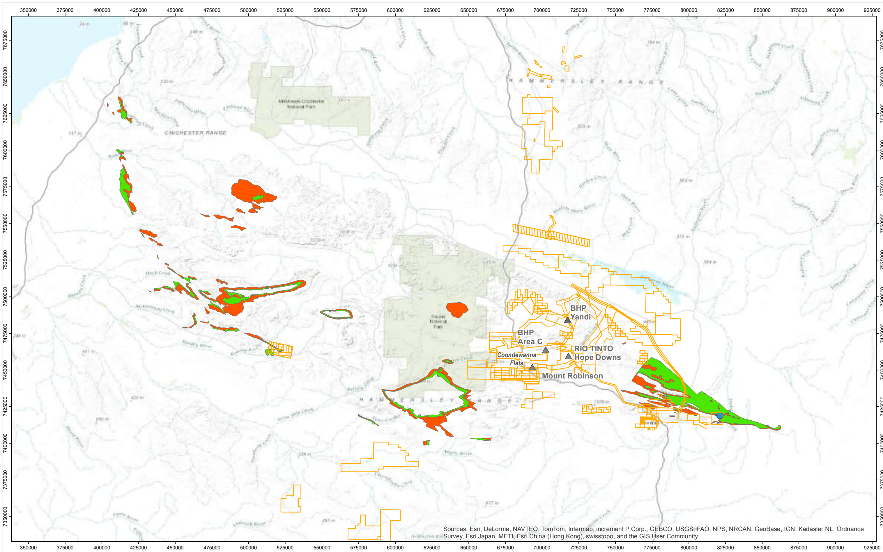
BHPBIO FIGURE 2 Distribution of the Boolgeeda Iron Formation and Woongarra Rhyolite
