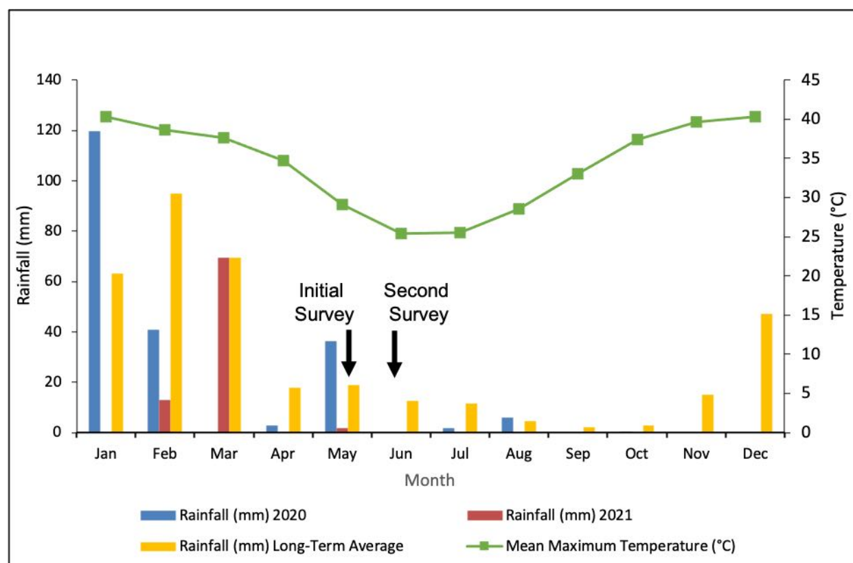
Figure 3. Monthly (2020-2021) and Long-Term Average Rainfall (mm); and Mean Maximum Temperature (°C) (Telfer) (Bureau of Meteorology 2021).
