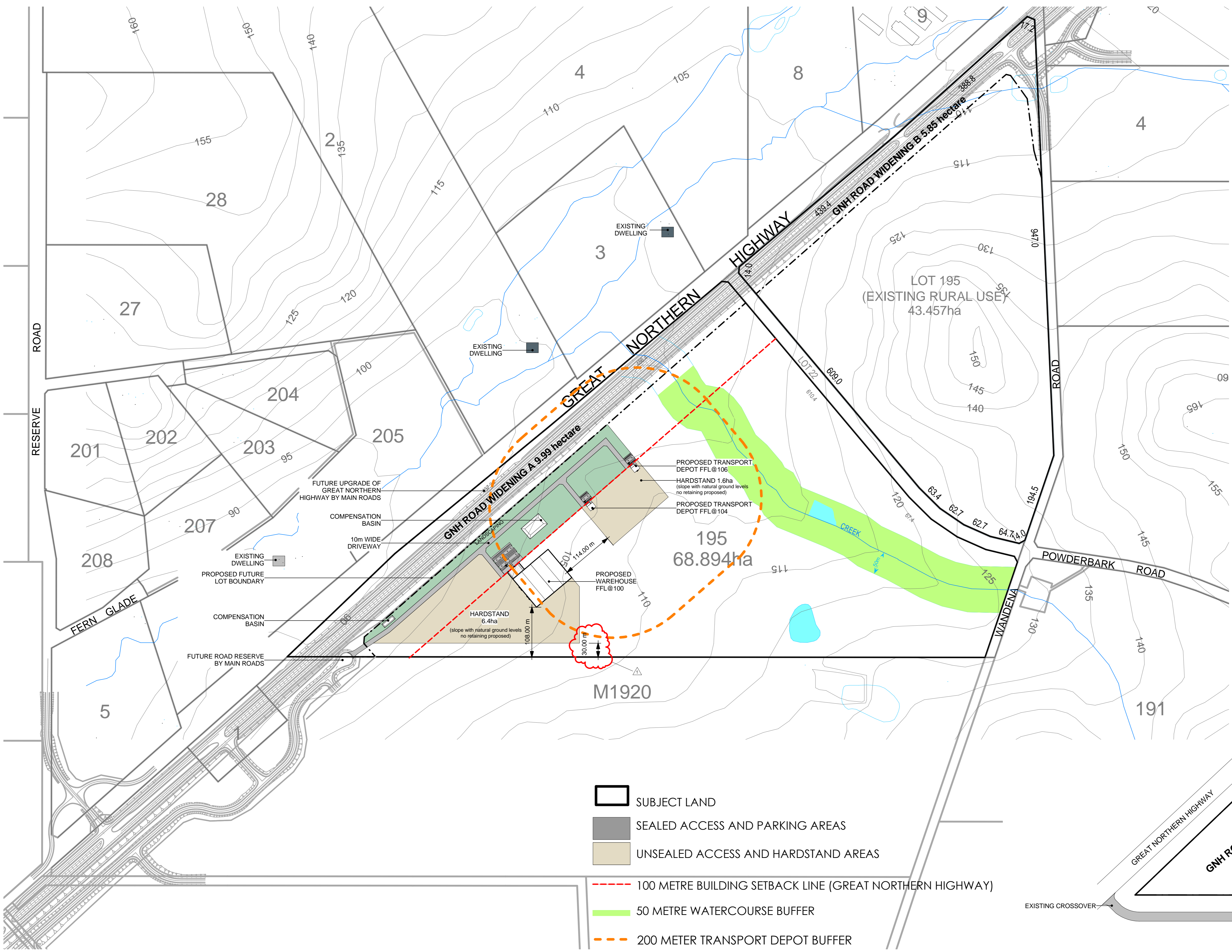
0 PROPOSED SITE DEVELOPMENT PLAN SCALE 1:4000
