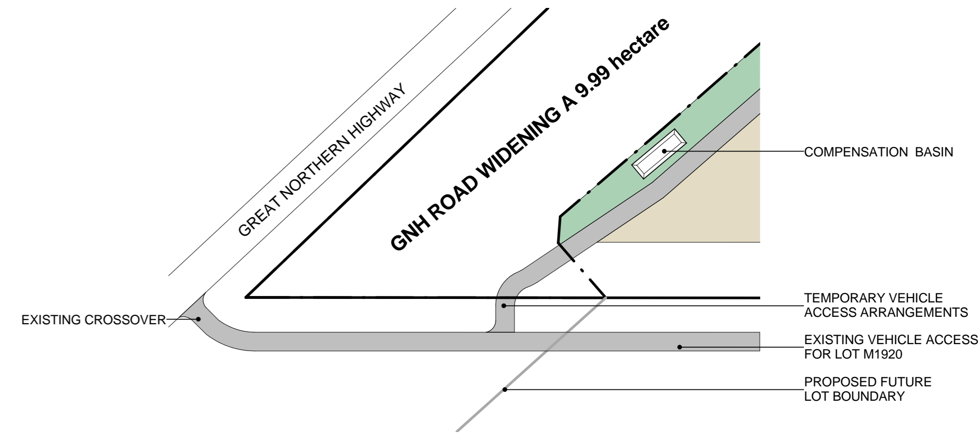
2 TEMPORARY ACCESS ARRANGEMENT SCALE 1:2000
