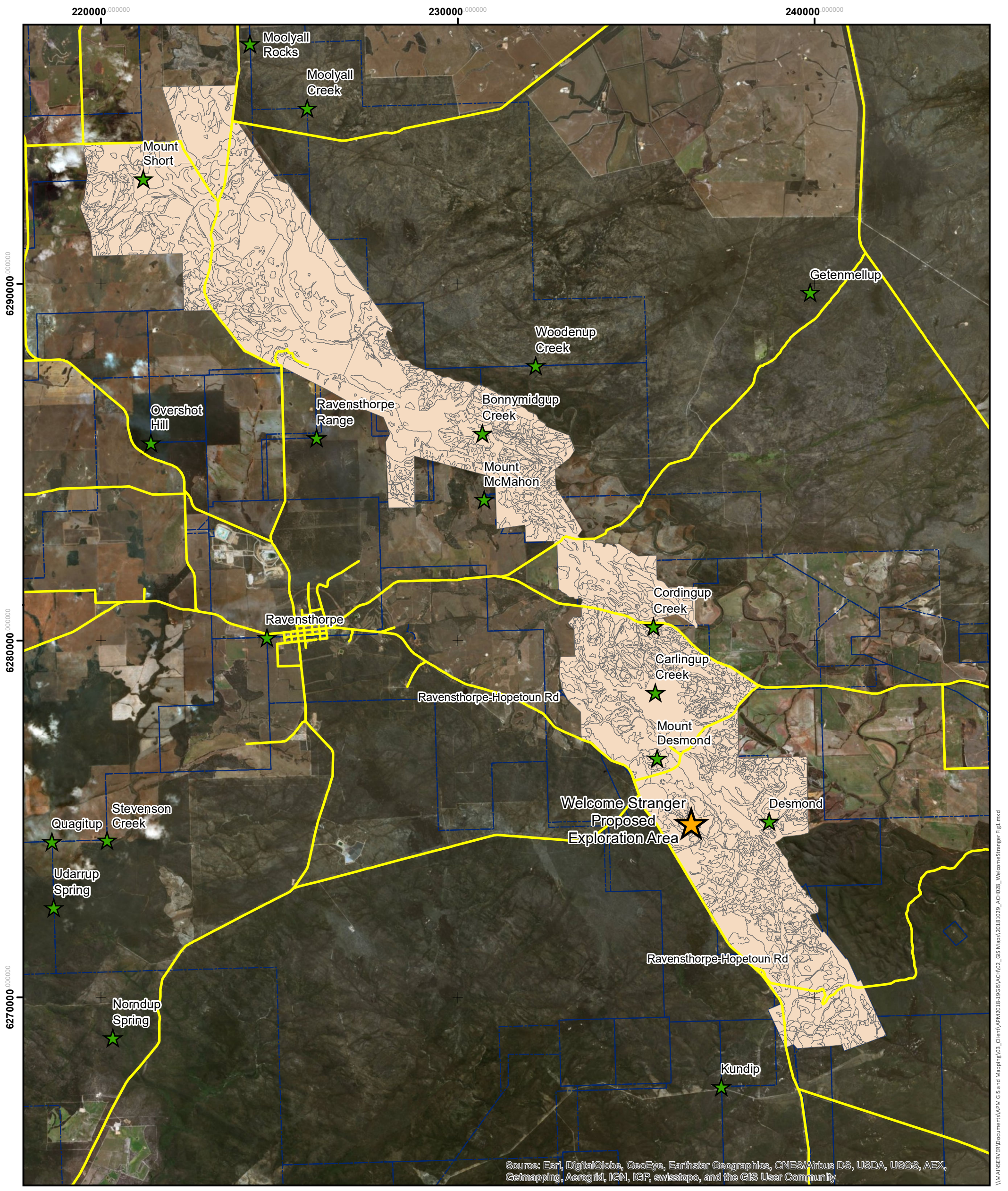
Figure 1: Locality of proposed Welcome Stranger exploration area in relation to Craig mapping of Ravensthorpe Range
